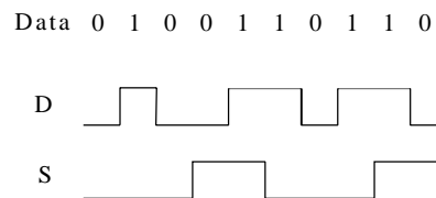
Figure 1 : Data-Strobe (DS) Encoding
