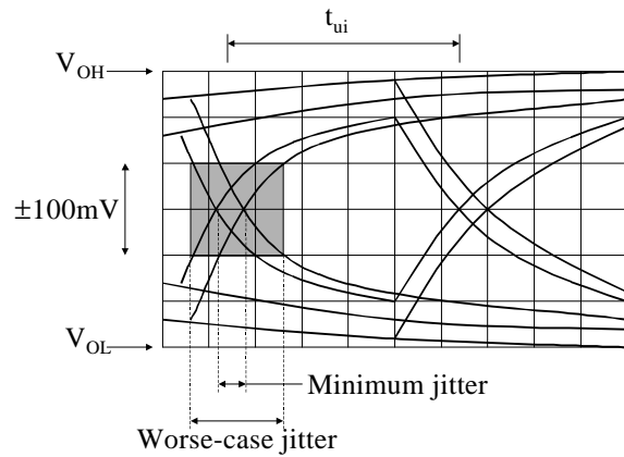
Figure 6 : Worse-Case Jitter Measured with Eye Pattern
