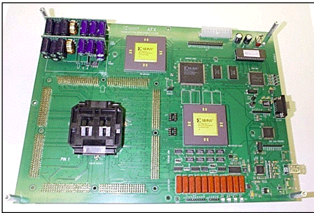
Figure 1: AFX motherboard used for SEE testing of the Virtex FPGA. Support circuitry interfaces to a PC and allows for configuration of the test device to a specific pattern or functional design.
