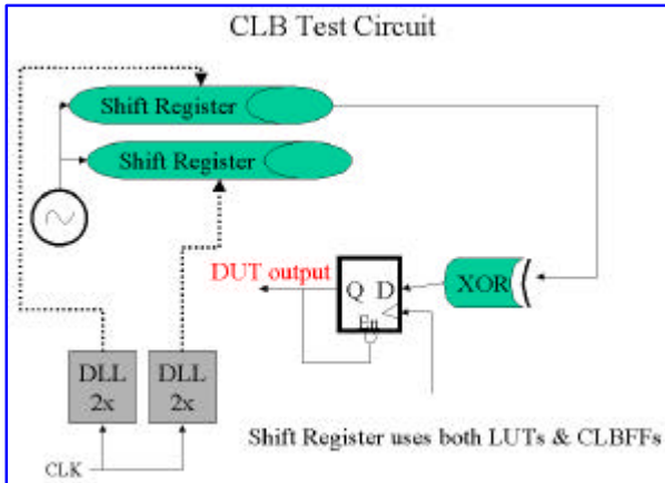
Figure 3: Configuration Logic Block dynamic test circuit.
