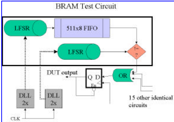
Figure 2: Block RAM dynamic test circuit.
