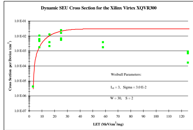
Figure 5: The device upset cross-section vs. LET for the Xilinx Virtex XQVR300 operating in a dynamic mode. The Weibull curve does not fit the data points well for LET values above 25. This is likely due to the method of measuring fluence to the first failure. The ion beam operator was required to manually respond to an error indicator and terminate the beam. With total beam exposure times of 2 to 3 seconds, the response time added significant error to the fluence applied.
