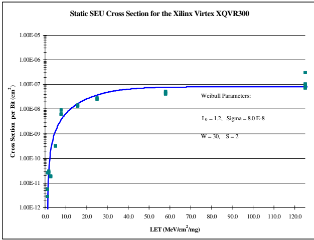
Figure 4: The bit upset cross-section vs. LET for the Xilinx Virtex XQVR300 for static operation.
