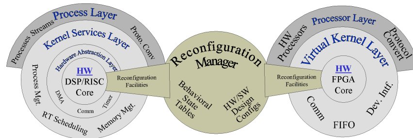
Figure 1. Runtime architecture
