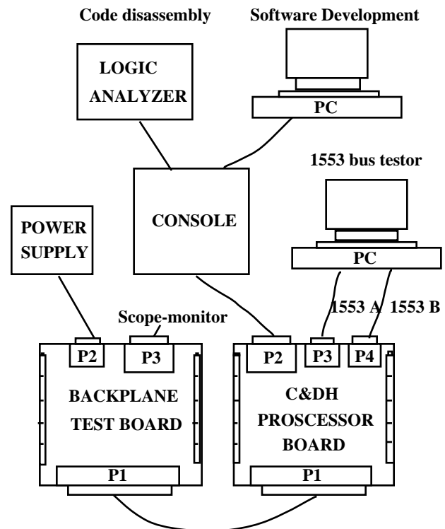
Figure 2. Test setup.
