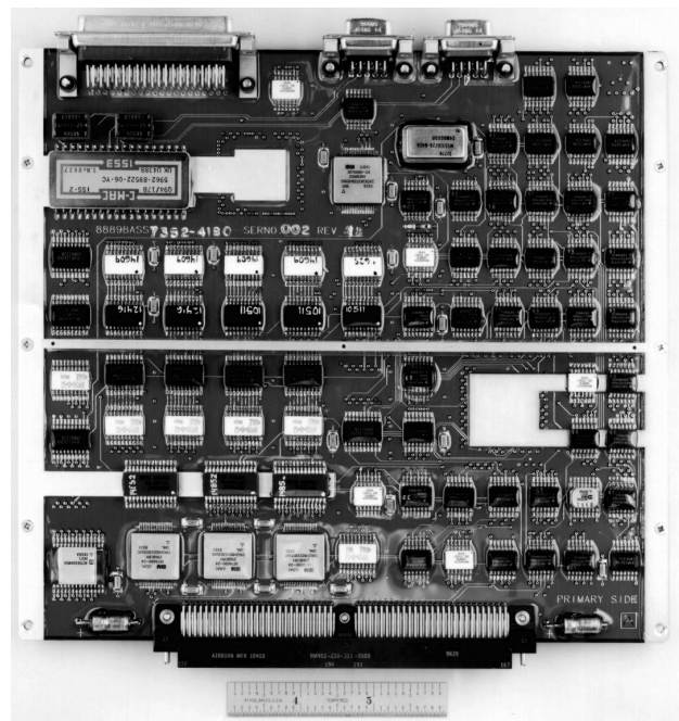
Figure 3. Circuit board front.
