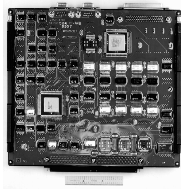
Figure 4. Circuit board back.
